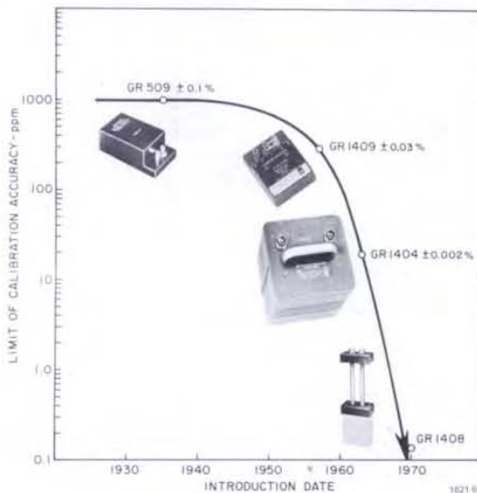
Figure 1. GR standard-capacitor calibration-accuracy improvement with time.
