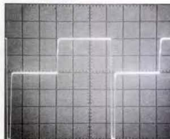
Figure 1. Programming pulse triggers trace of attenuation transition from 0 dB to 40 dB at 30 MHz. Horizontal scale: 1 ns/cm. Vertical scale: 10 dB/cm.
