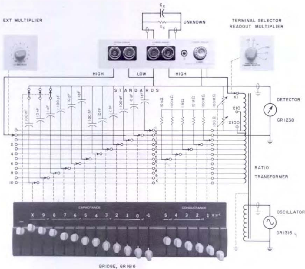
Figure 9. GR 1616 bridge: Basic circuits.
