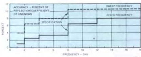
Figure 4. RF-unit accuracy.
