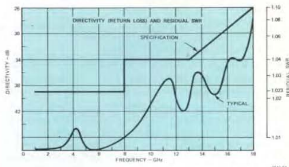
Figure 1. RF-unit directivity.
